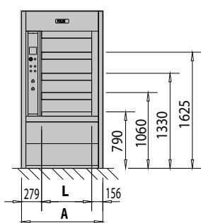
Mod. 62-4 Chambers
