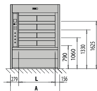
Mod. 124-4 Chambers
