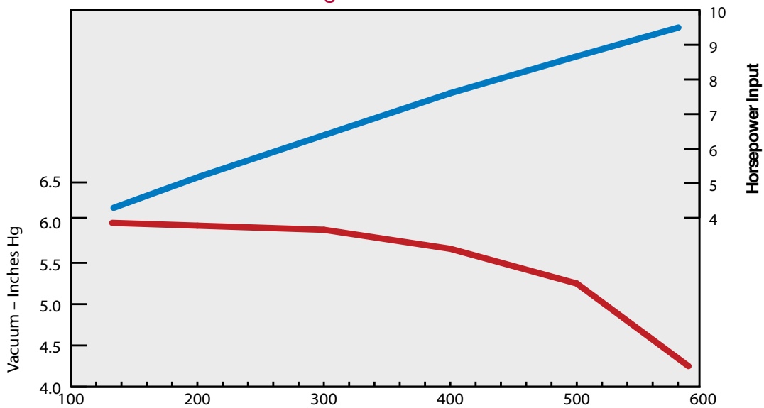
Chart 4 Gardner Denver Performance Curve Model 407 Atmosphere Conditions 29.92 inches Hg 68°F
