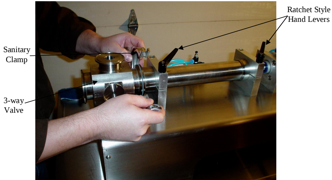
Figure 5-3 Disassembly
