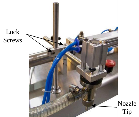
Figure 5-10 FPT Series Fillhead
