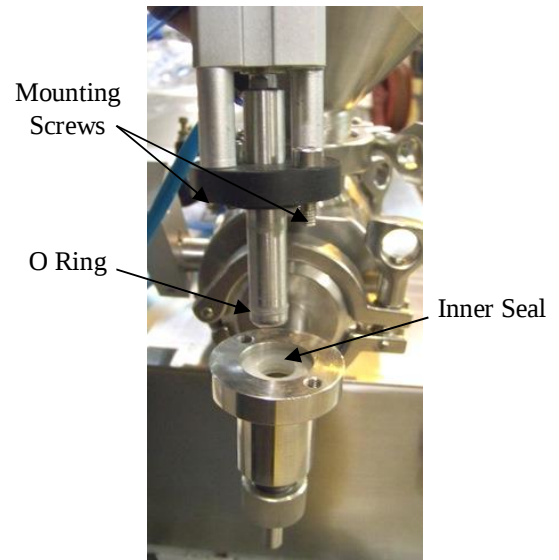
Figure 5-13 Bottom Close Nozzle Cylinder
