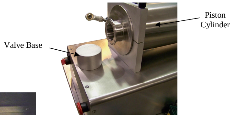
Figure 5-4 Valve Base
