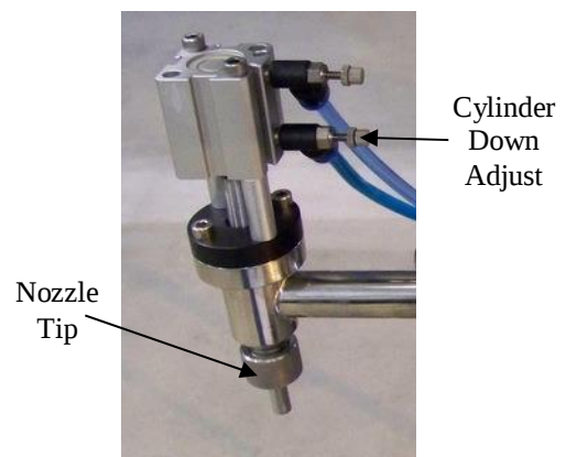
Figure 4-4 Bottom Close Nozzle
