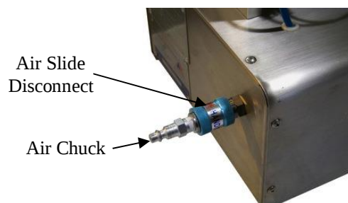
Figure 3-5 Air Inlet
