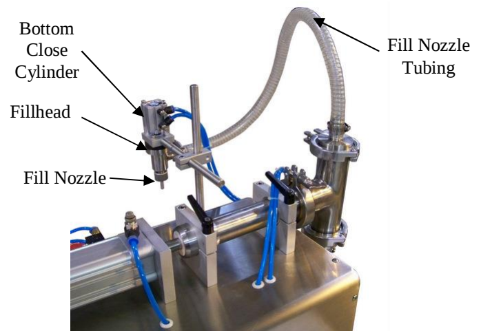
Figure 3-2 FPT Series Fillhead
