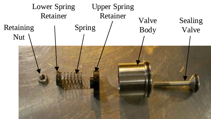
Figure 5-11 Fill Check Valve Disassembled
