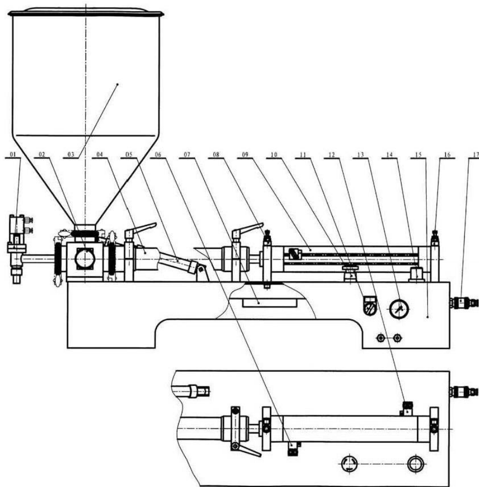
FPV FILLER DRAWING
