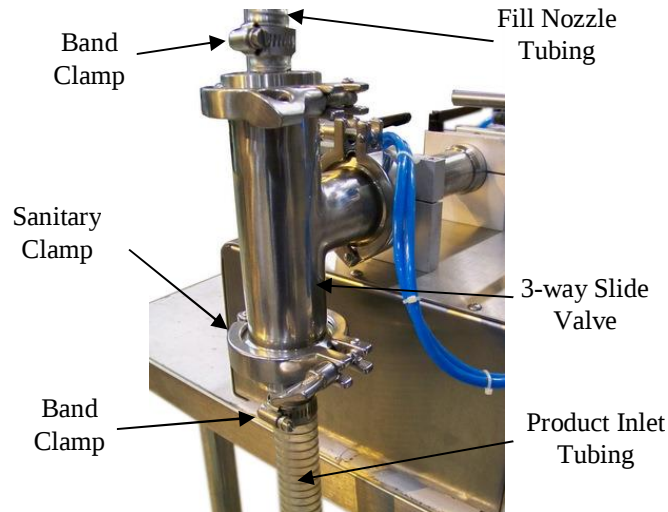
Figure 3-1 3-way Slide Valve Inlet
