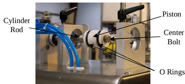
Figure 5-5 Piston
