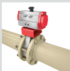
High performance double offset butterfly valve (> 2" NPT)
